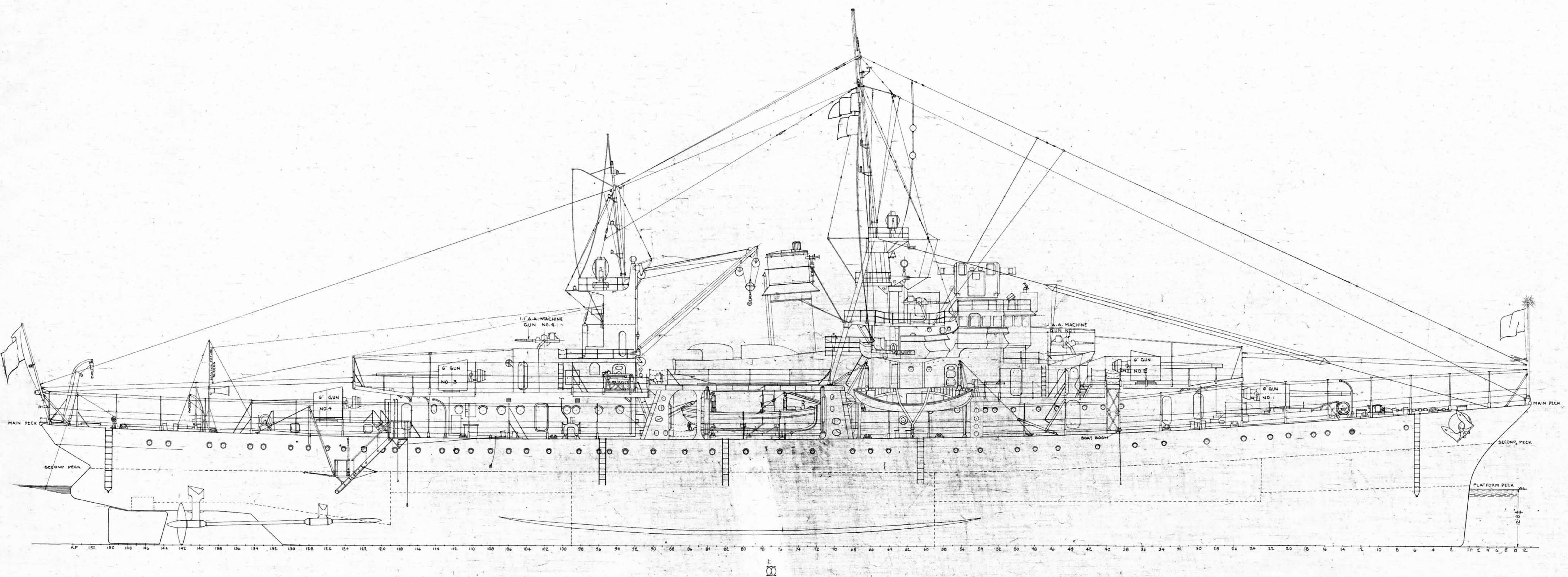
OUTBOARD PROFILE
